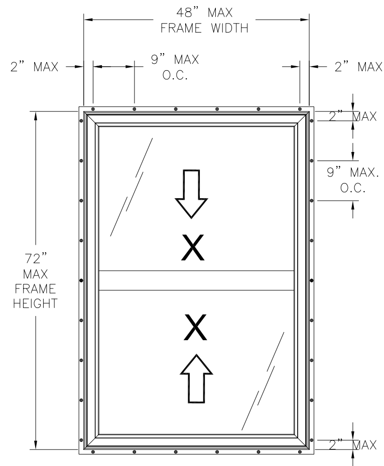
S-SERIES DOUBLE HUNG EXTERIOR VIEW FIN INSTALLATION
